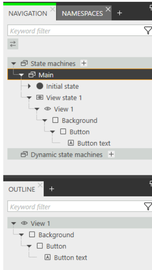
Figure 1. Widget hierarchy
