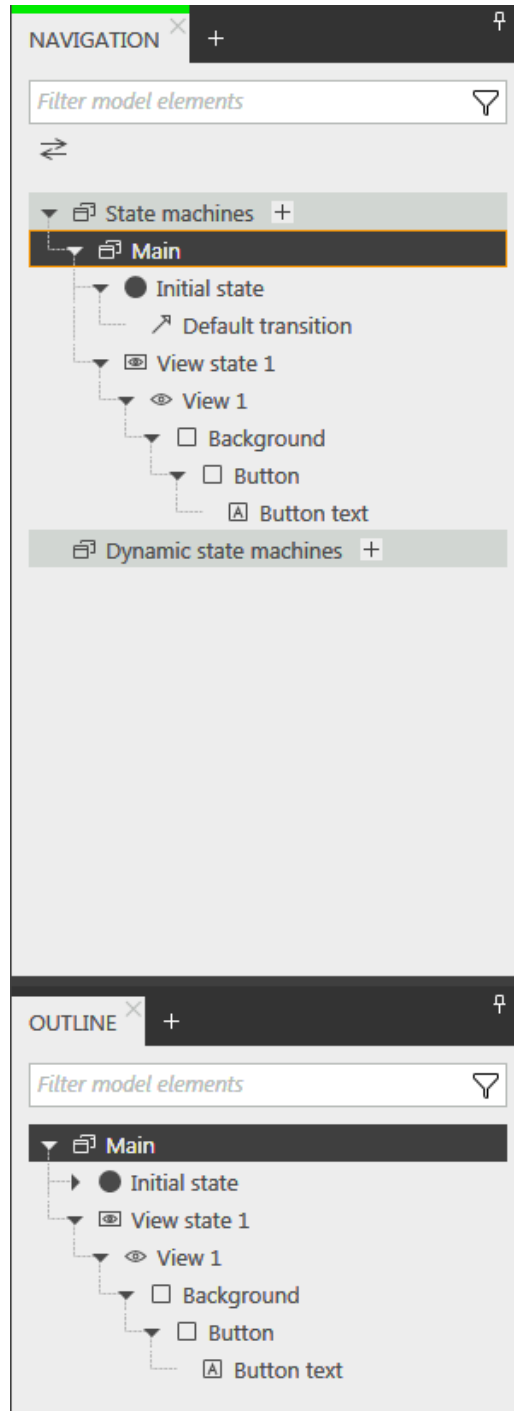
Figure 1. Widget hierarchy
