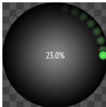
Figure 5.3. TL_Progressbar_Radial
