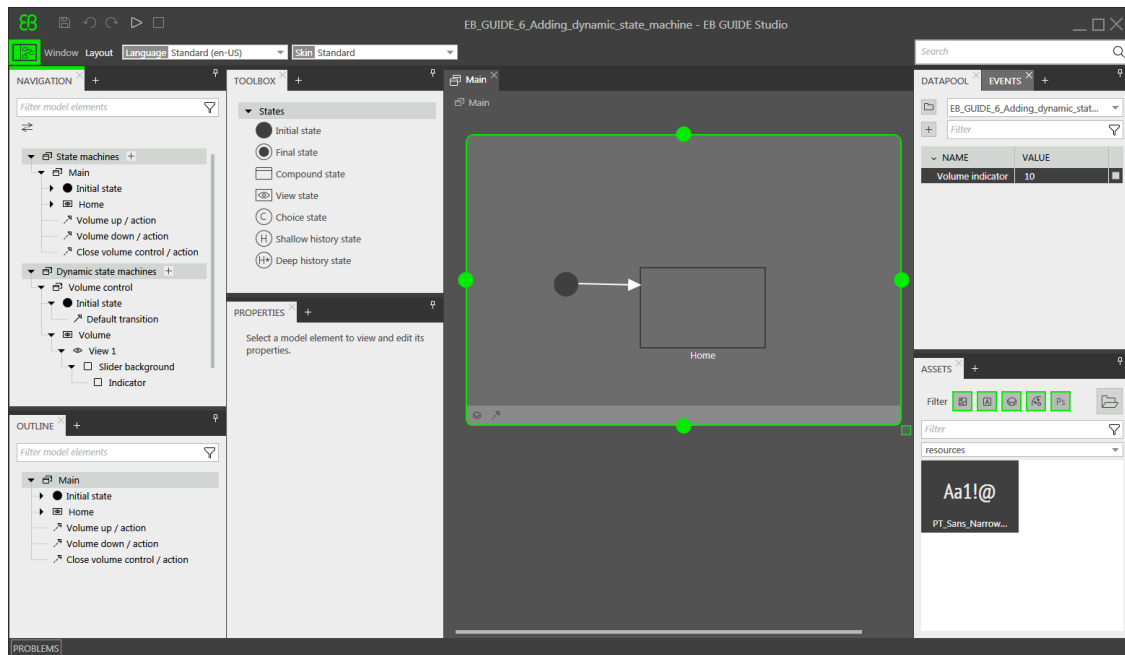
Figure 2. EB GUIDE model with all model elements
